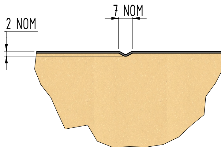
DETAIL A
